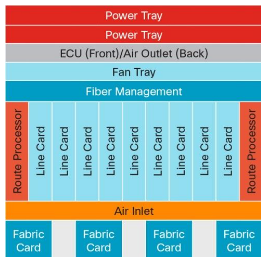
Figure 4. Cisco NCS 4009 Shelf Architecture
