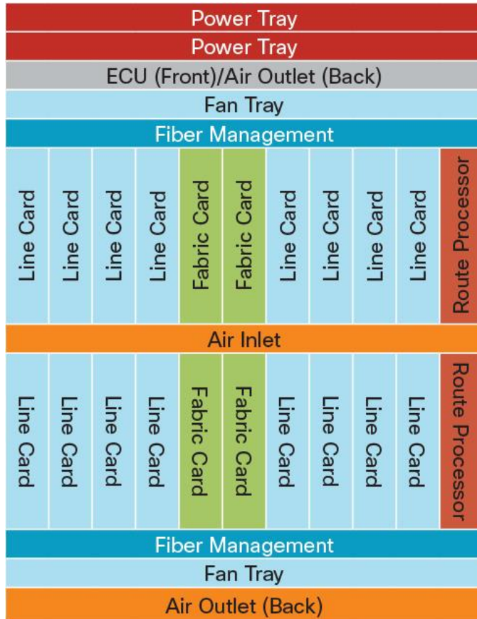
Figure 2. Cisco NCS 4016 Shelf Architecture
